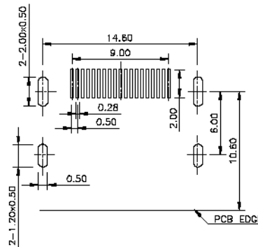
PCB RECOMMENDED LAYOUT (TOP VIEW) Tolerance ±0.05
