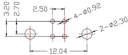
PCB BOARD LAYOUT
